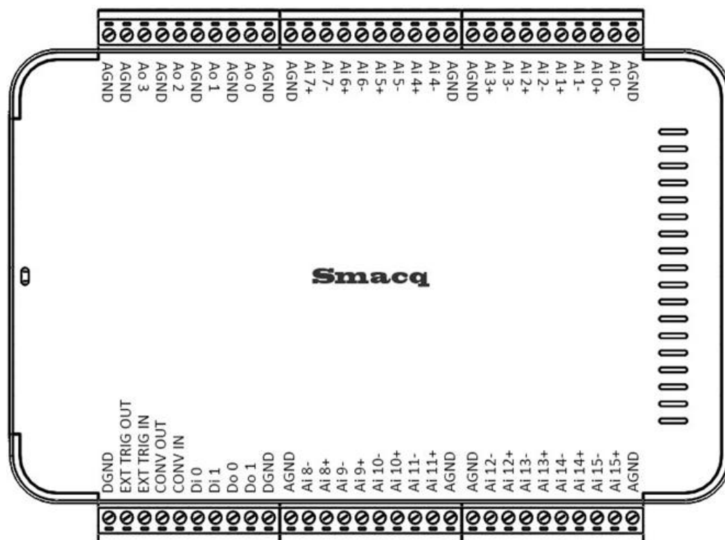
USB-5700 signal pins distribution
