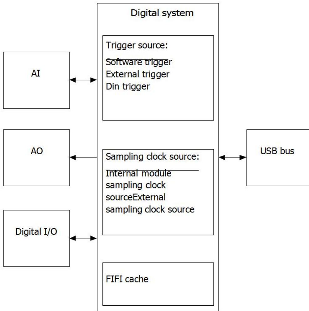
USB-5700 series data acquisition device functions schematic
