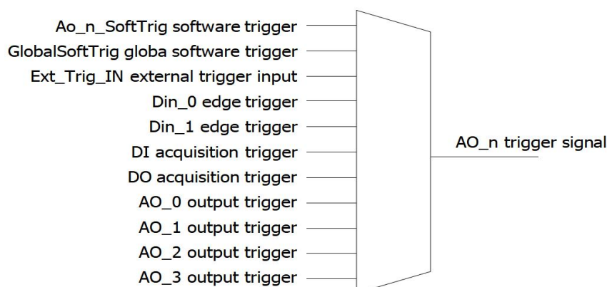
Trigger options for an AO output channel
