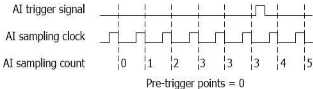
AI pre-trigger function diagram
