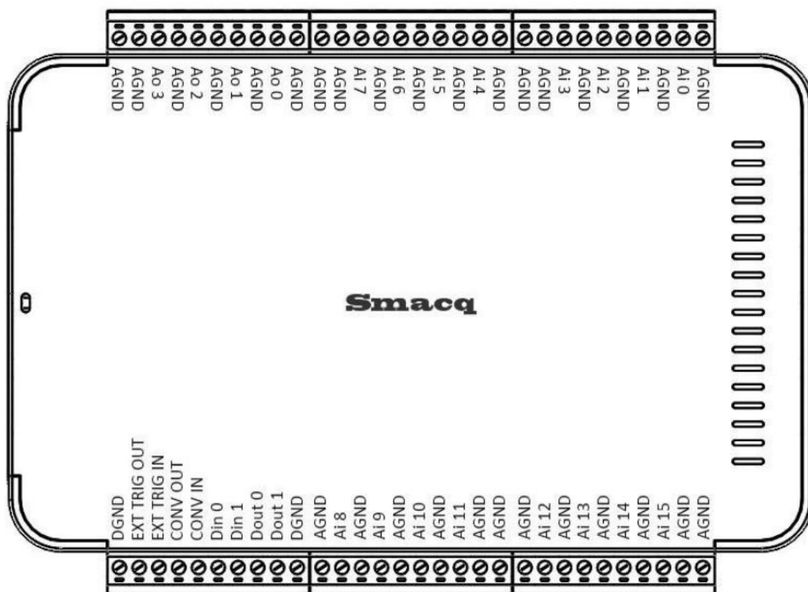
USB-5200 series signal pins distribution
