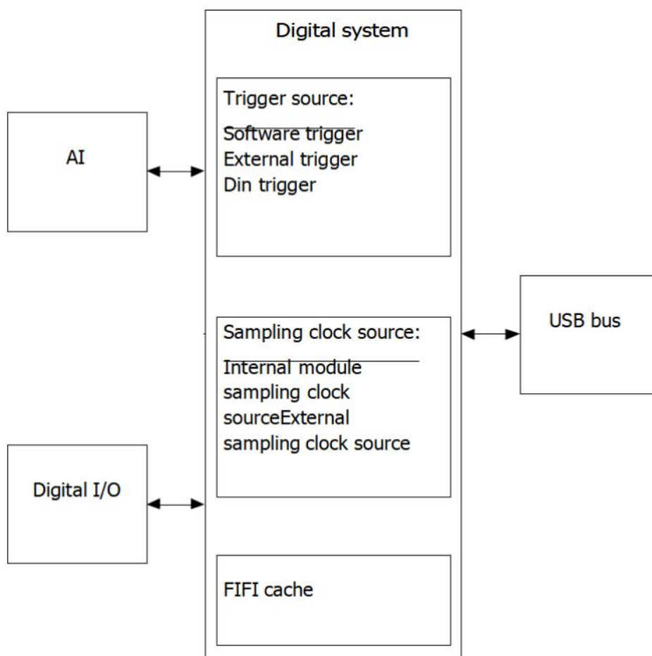
USB-5200 series data acquisition device functions schematic
