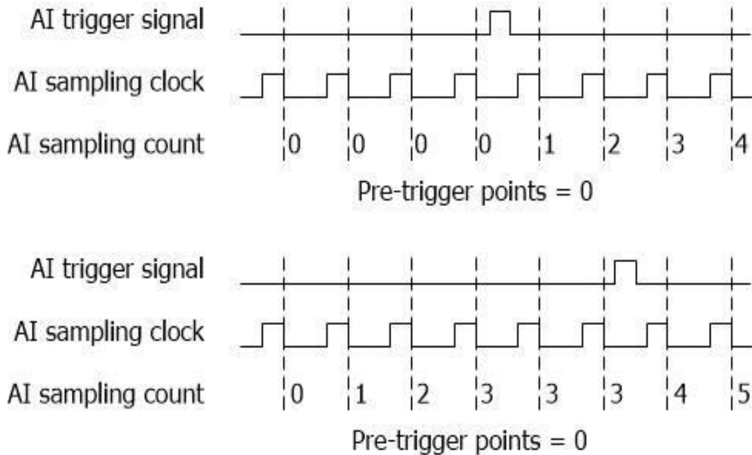
AI pre-trigger function diagram
