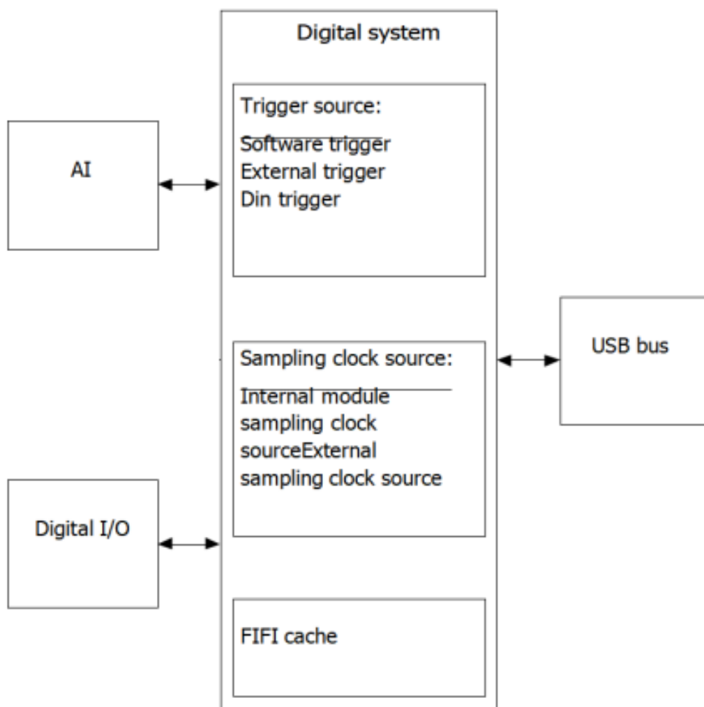
USB-3200 series data acquisition device functions schematic
