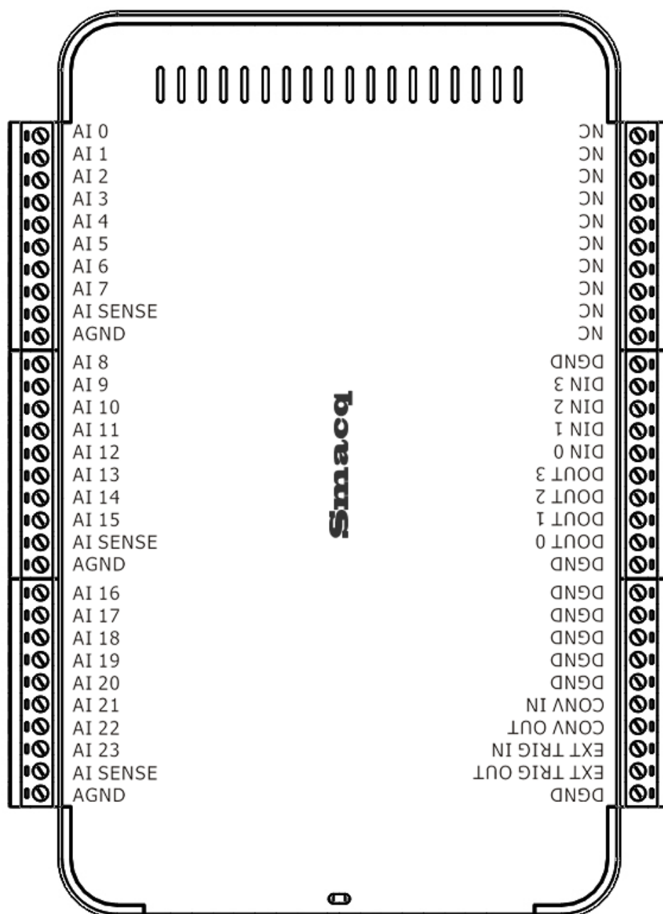
USB-3200 series signal pins distribution
