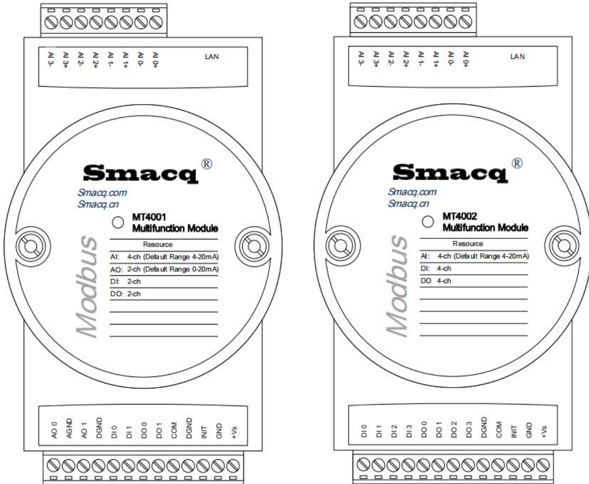
MT4000 Wiring Definition
