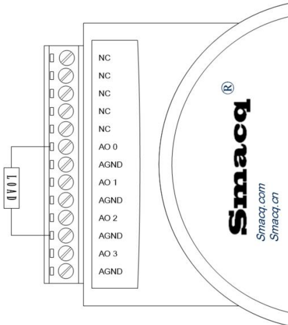
Schematic diagram of current signal analog output connection
